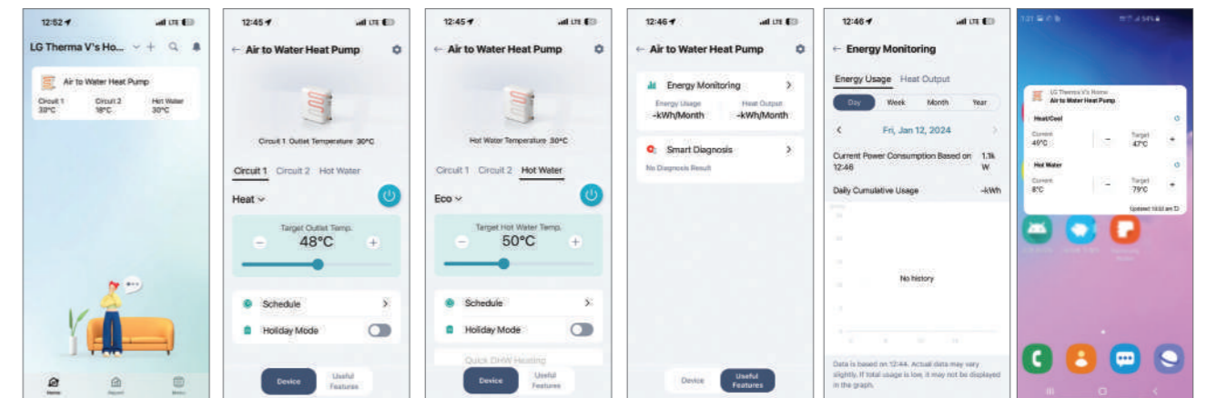
Home screen
